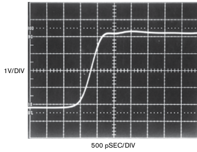
Figure C Figure B 's pulse viewed with a Tektronix low-impedance 500\Omega P-6056 probe introduces barely discernible error.
