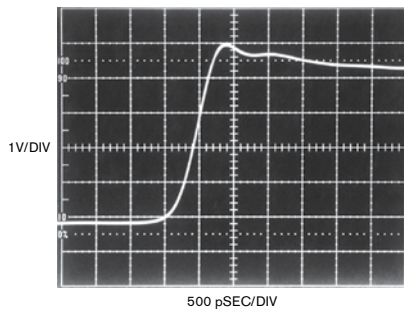
Figure E Do-it-yourself Z_0 Probe 2 has overshoot, again likely due to resistor/cable parasitic terms or incomplete coaxiality. At these speeds, don't do it yourself.
