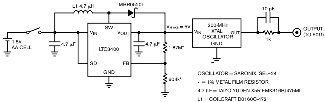
Figure A A 1.5V-powered, 200-MHz crystal oscillator provides 5-nsec time markers. A switching regulator converts 1.5 to 5V to the power oscillator.
