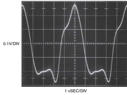
Figure B A time-mark generator output terminates into 50\Omega . A peaked waveform is optimal for verifying time-base calibration.
