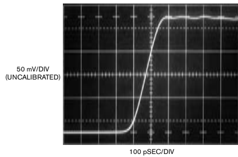
Figure C A 20-psec step produces an approximately 140-psec probe/oscilloscope rise time.
