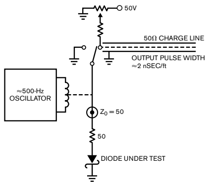
Figure A When right-side contacts close, the charge line discharges into a 50Ω diode load. Strict attention to construction allows wideband, 50Ω characteristics, permitting a 250-psec rise time and a high-purity output pulse.
