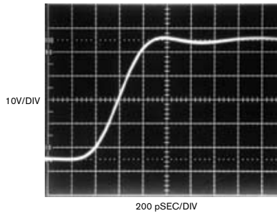
Figure B Tektronix type 109 produces a high-purity, 50V, 1A pulse, driving the monitoring 1-GHz oscilloscope to its 350-psec-rise-time limit.
