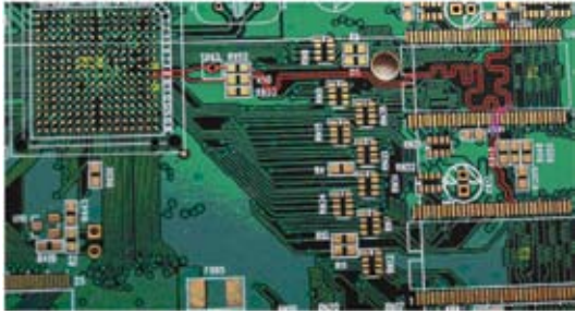
Figure 2 The bare PCB shows the differential-signal traces from the SOC to IC 1 and IC 2 .
