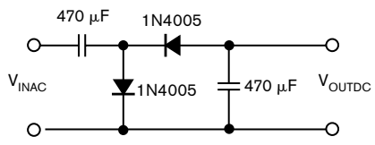
Figure 2 A conventional voltage doubler uses diodes.
