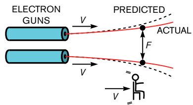
Figure 1 The electric force between two charged particles makes their trajectories diverge.
