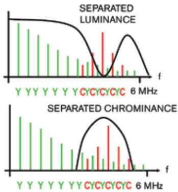
Figure 3 Notch filters and bandpass filters separate the luminance and the chrominance.
