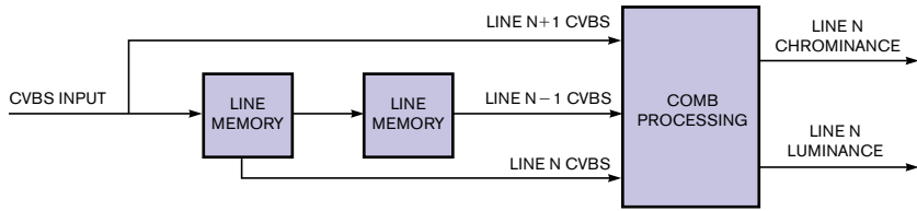
Figure 6 A three-line, 2-D comb would introduce a one-line delay from input to output.
