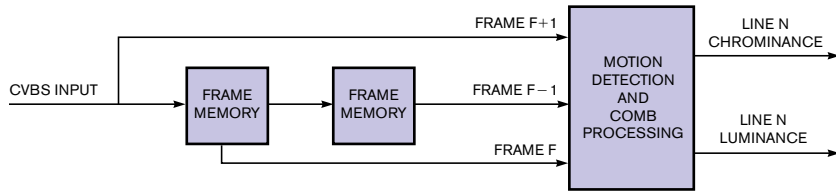
Figure 7 A typical 3-D-comb decoder architecture supplements the previous-generation 2-D comb's spatial implementation with added temporal cognizance.
