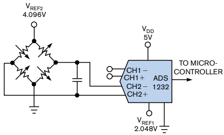
Figure 2 A 24-bit load-cell system has greater-than-0.25-lb accuracy.
