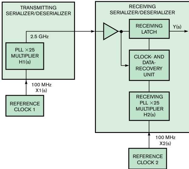
Figure 3 The PCIe separate-clock architecture employs a second reference clock in the receiver.
