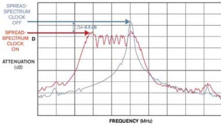
Figure 4 Spread-spectrum clocking can reduce EMI peaking to meet system-emissions limits.
