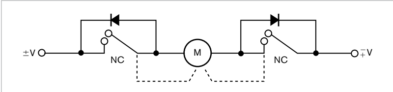
Figure 1 This circuit works by inhibiting movement in one direction but allowing movement in the other direction when the motor retracts from its end position.
