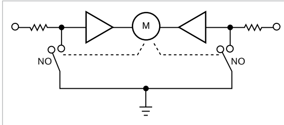
Figure 2 This circuit shortens one input of the H bridge to ground so that movement is possible only in the other direction by turning on the other input.
