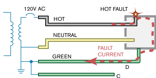
Figure 2 The green wires prevent the faulty chassis from remaining energized but do not prevent large voltages from appearing between points C and D.
