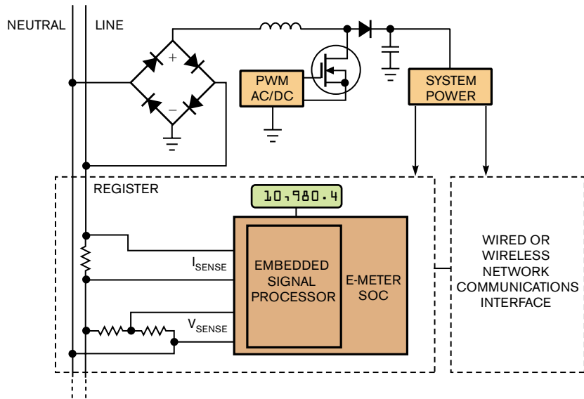
Figure 1 Smart power meters comprise a microcontroller with onboard ADC and DAC, a sensing component for both voltage and current, an ac/dc-power converter, battery backup, and wireless or wired communication capability.
