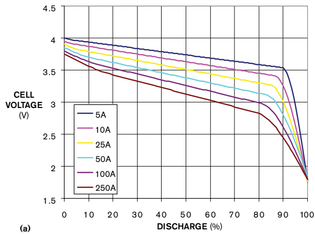
Figure 1 The charge-versus-voltage characteristics of a typical 5A-hr lithium-ion cell are shown at various discharge rates (a). The charge-versus-voltage characteristics for the same cell at various temperatures are shown during a 5A discharge (b).
