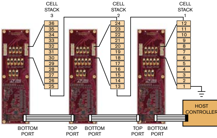
Figure 3 You can monitor a representative 36-cell pack in three groups of 12 cells each. The 12-cell module supplies local power and ground to the analog electronics. By breaking the stack into small groups, the analog circuits see a much smaller common-mode voltage.
