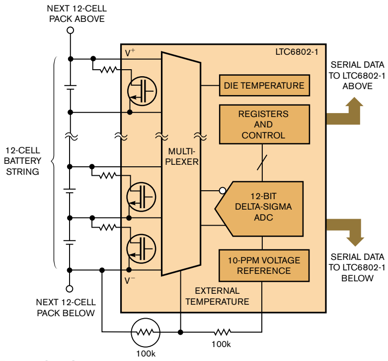
Figure 5 One IC integrates most of the functions in a simplified cell-measurement design.
