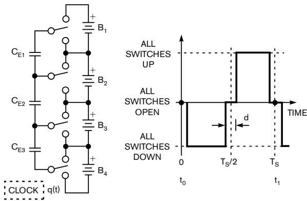
Figure 9 This capacitor-based scheme uses a capacitor that continuously switches between two adjacent cells. Current flows to equalize the voltage and, therefore, the state of charge of the two cells. Active balancing shuttles charge between cells and does not become wasted heat. It requires a storage element for the charge transfer.
