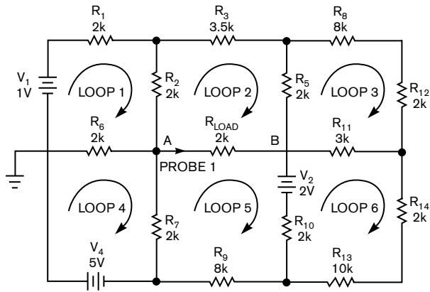
Figure 2 The simulation for current through the load resistance yields -60.3 \mu\text{A} .
