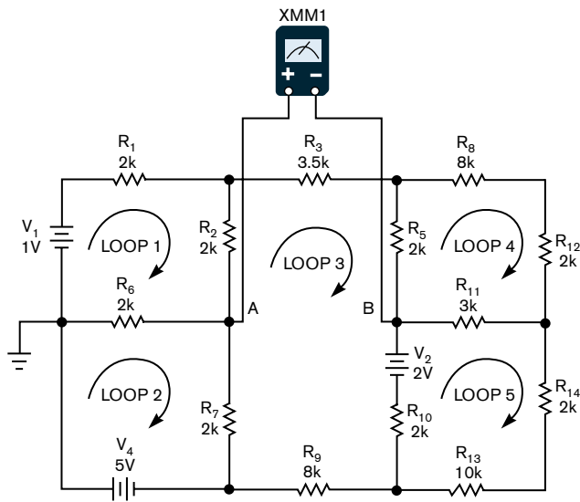
Figure 3 The simulation for the open-circuit voltage yields approximately -374 mV.
