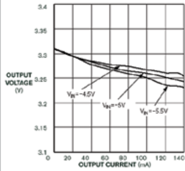
Figure 2 The circuit's output voltage drops as current increases. Plots indicate source voltages of -4.5 , -5 , and -5.5V .
