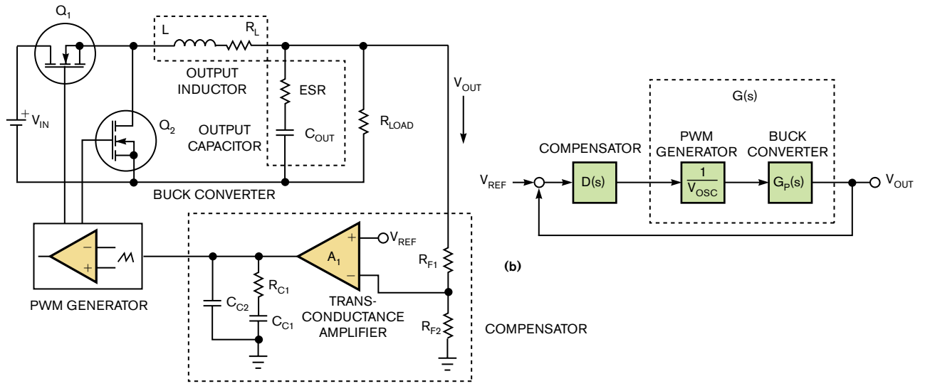
Figure 2 Taking a typical buck regulator circuit—shown here in circuit (a) and block-diagram (b) form—you solve for G(s) : G(s) = D(s) \times G_p(s) .
