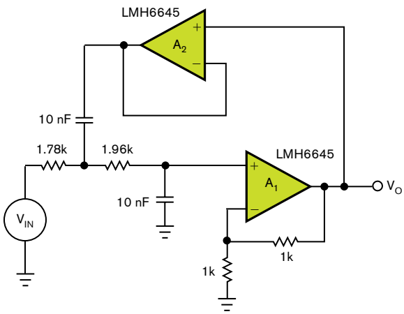
Figure 7 The experimental filter uses 55-MHz voltage-feedback amplifiers.
