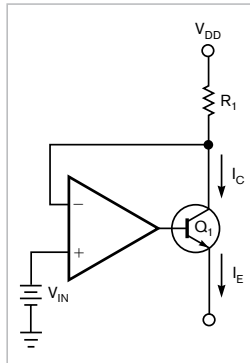
Figure 1 The voltage-to-current converter relies on the fact that the collector current is approximately equal to the emitter current and provides current in only one direction.
