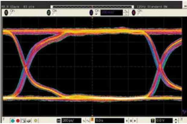
Figure 3 With the optimal termination value, driver impedance, and output inversion enabled, the postregister DDR3 data-eye plot exhibits a wider opening with minimal ring-back.
