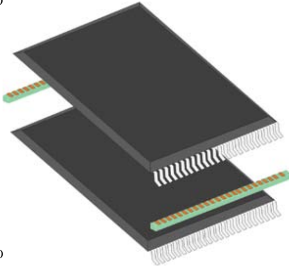
Figure 7 You can use a flex circuit and a PCB interposer to stack BGA (a) or TSOP (b) DRAM.
