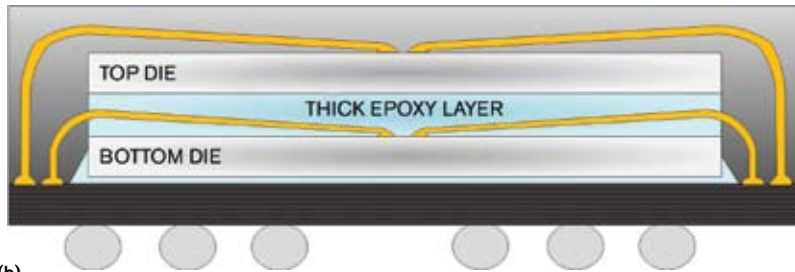
Figure 8 One version of die-stack-packaging technology has an interposer (a); another version does not (b).
