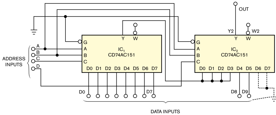
Figure 1 The maximum worst-case propagation delay of this 10-line-to-one-line data selector/multiplexer is 27 nsec, whereas the typical value is only 6.8 nsec. The circuit can also serve as a 12-to-one multiplexer.
