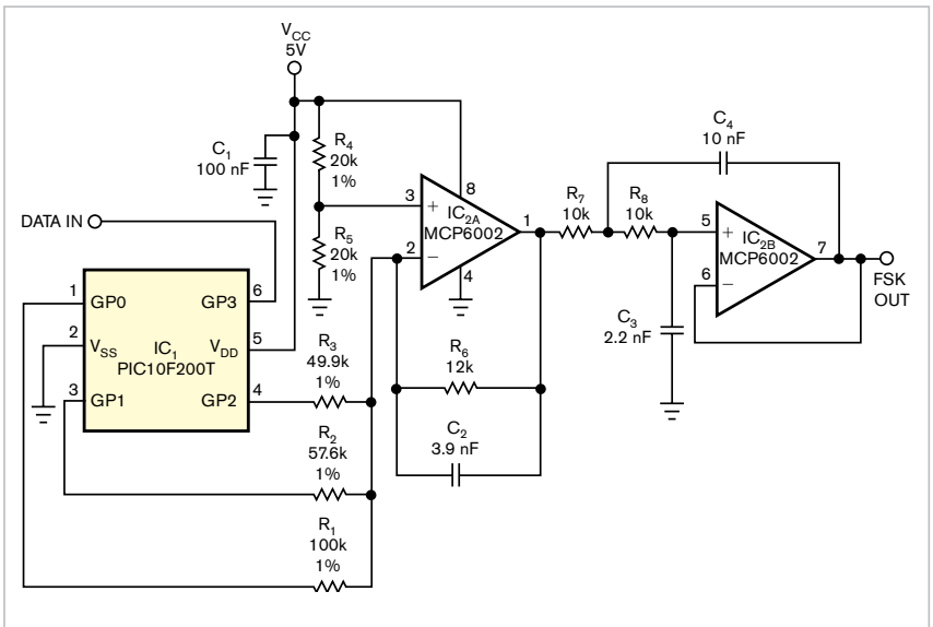
Figure 1 This microcontroller-based circuit generates Bell 202-compatible FSK modulation.
