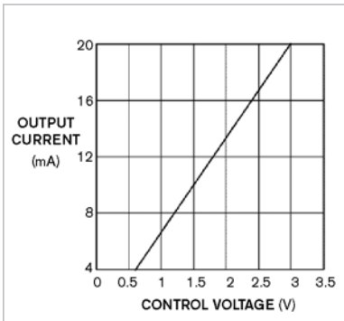
Figure 2 The circuit in Figure 1 produces a linear output current versus digital control voltage.
