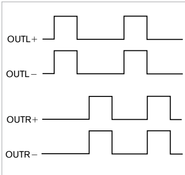
Figure 2 The MAX9704 applies power to one channel at a time.
