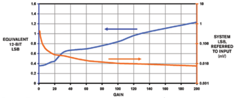
Figure 2 The system accuracy is better than 0.01% with PGA gains of 1 to 125V/V. With PGA gains of 125 to 200V/V, the system accuracy is better than 0.02%.
