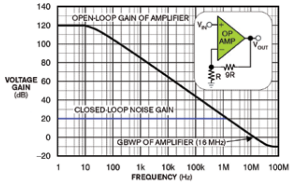
Figure 1 The open- and closed-loop gain of this voltage-feed-back amplifier has a gain-bandwidth product of 16 MHz and a circuit noise gain of 10V/V.
