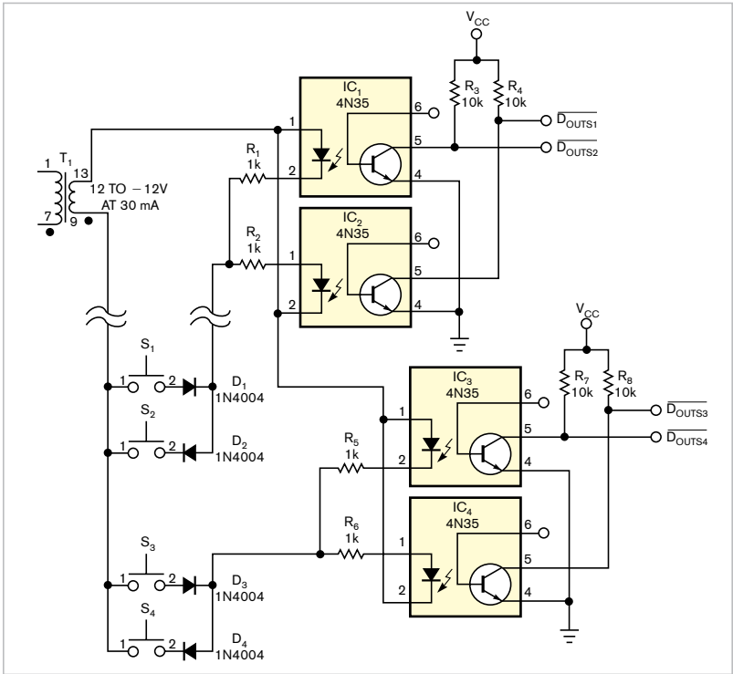
Figure 2 By adding a third wire, you can connect four pushbutton switches.
