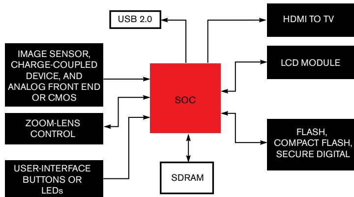
Figure 2 An SOC at the heart of a board may also be the best place to observe and control the outlying digital blocks.
