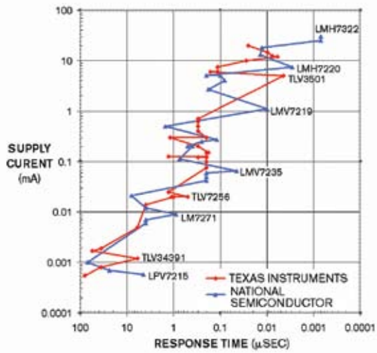
Figure 2 The faster a comparator switches, the more power it consumes.
