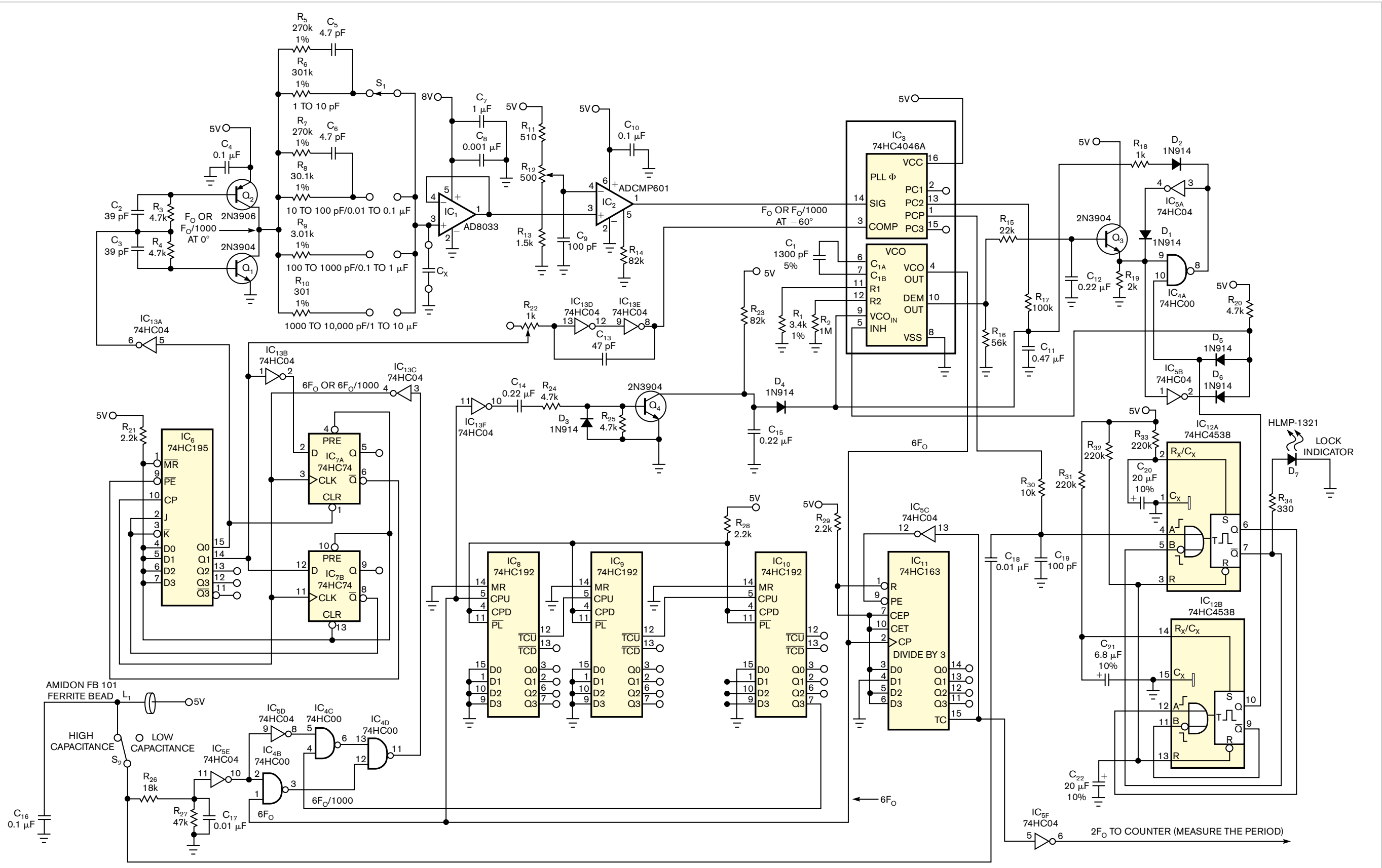
Figure 1 A capacitance meter connects to a frequency counter measuring pulse width to provide a capacitance measurement.
