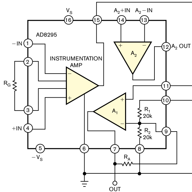
Figure 1 In this configuration, the first-order drift of the gain cancels, and the gain splits equally between the instrumentation amplifier and A_1 .
