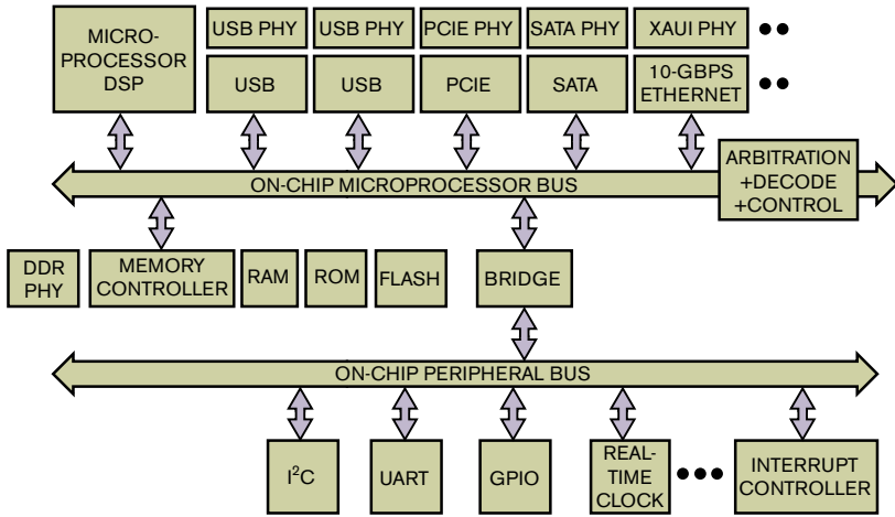
Figure 1 Standards-based IP may make up a significant portion of an SoC design.
