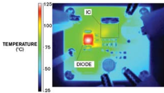
Figure 2 A thermal camera takes an image that shows hot spots on a PCB.
