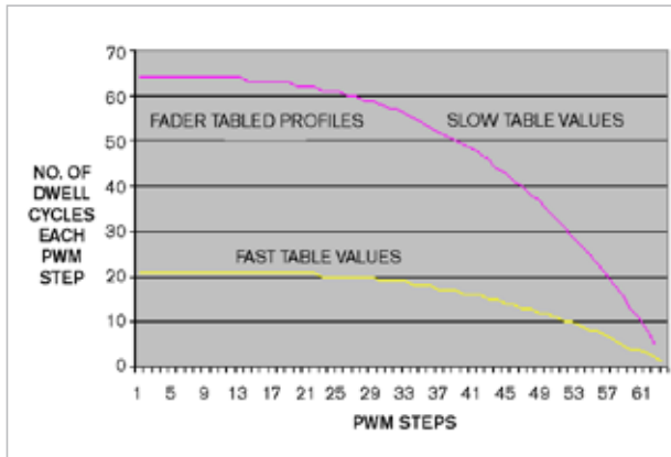
Figure 2 A table in the microcontroller code lets you run fast- or slow-fading profiles.
