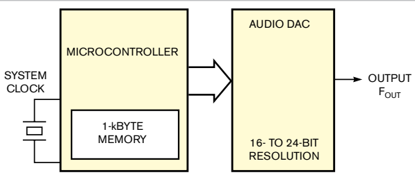
Figure 1 A microcontroller with a small memory can drive a DAC to generate audio-frequency signals.
