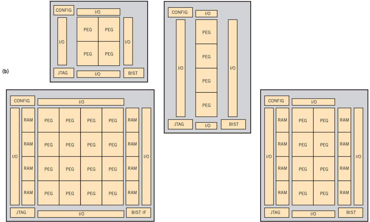
The elemental Actel logic cell (a) hierarchically multiplies to form programmable embedded-gate arrays of various shapes and sizes (b).
