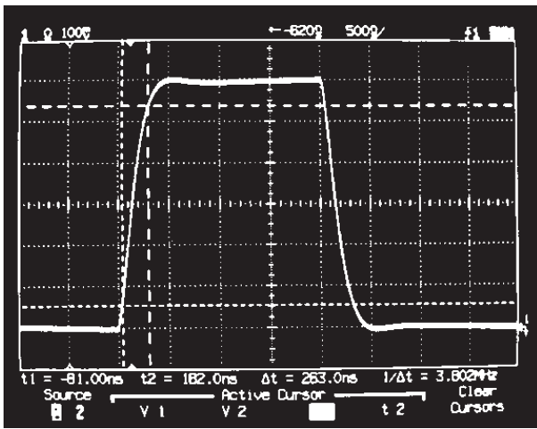
Figure 3 The circuit of Figure 2 exhibits clean pulse response with little overshoot or ringing.
